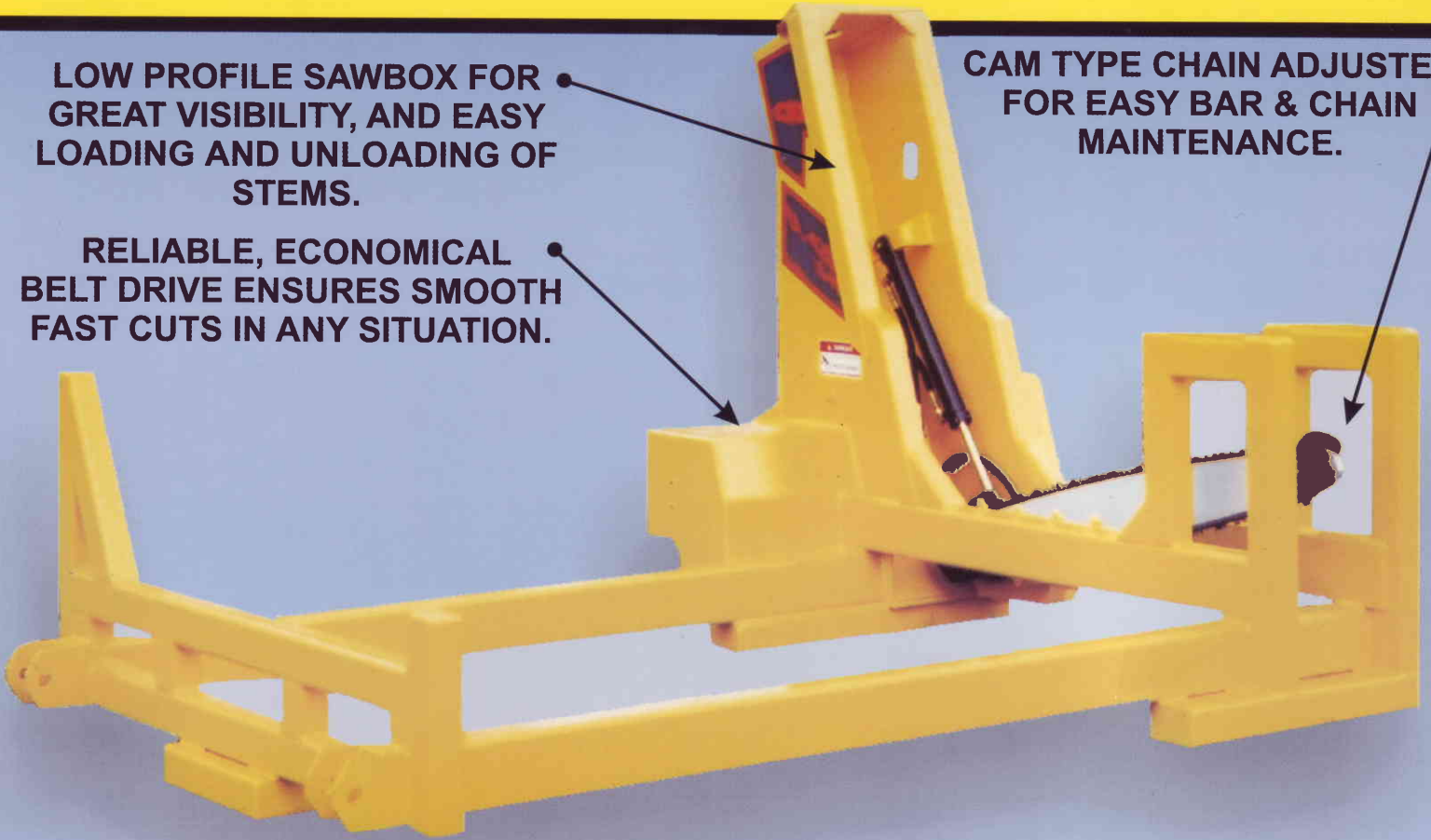
CSI MODEL DL-4200 LO-PRO-SLASHER SHOWN WITH STANDARD 8ft CHASSIS
